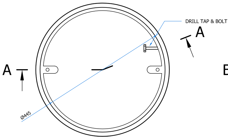
TOP VIEW OF FRAME
