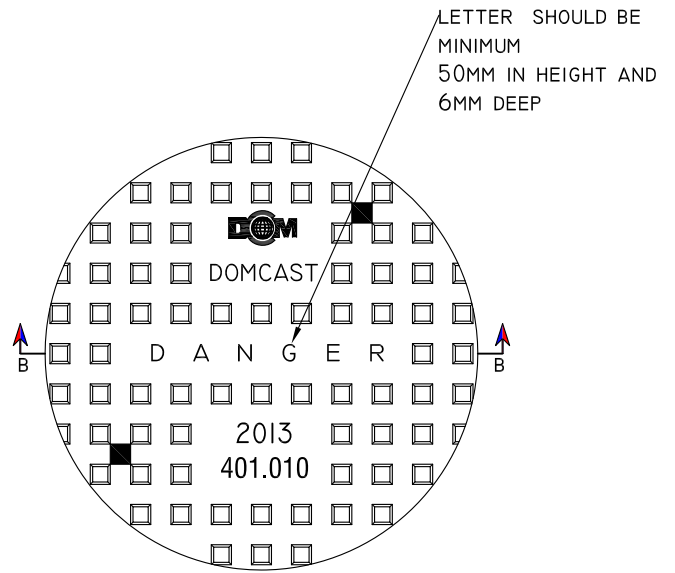
TYPE A CLOSED COVER
