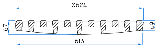
SECTION C-C
