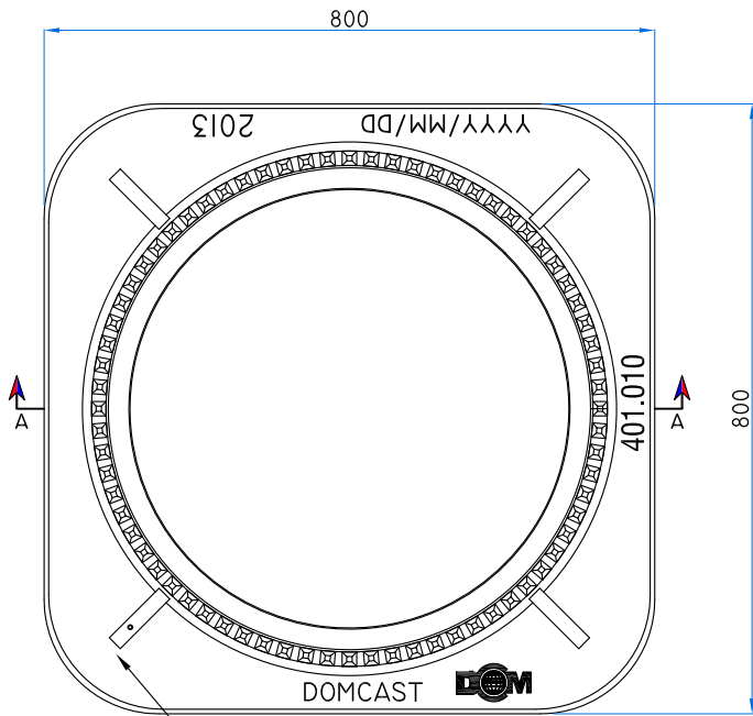
HOISTING HOOK RIB TYP. OPSD 400.001 FRAME PLAN
