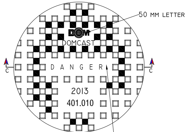
TYPE B OPEN COVER
