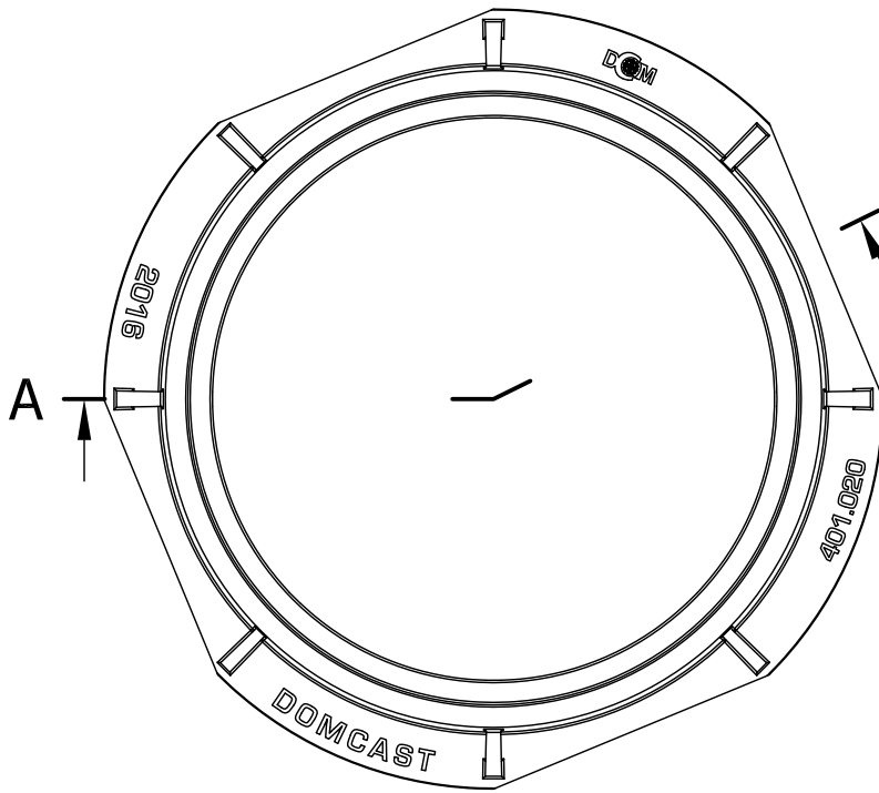
TOP VIEW OF FRAME
