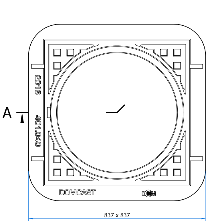
TOP VIEW OF FRAME
