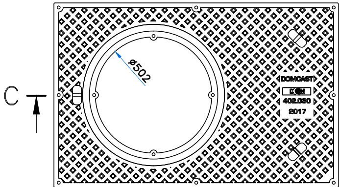
TOP VIEW OF RECTANGULAR COVER
