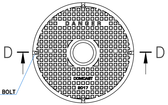
TOP VIEW OF CIRCULAR COVER
