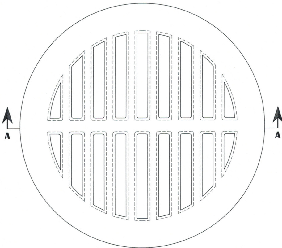
PLAN OF GRATE
