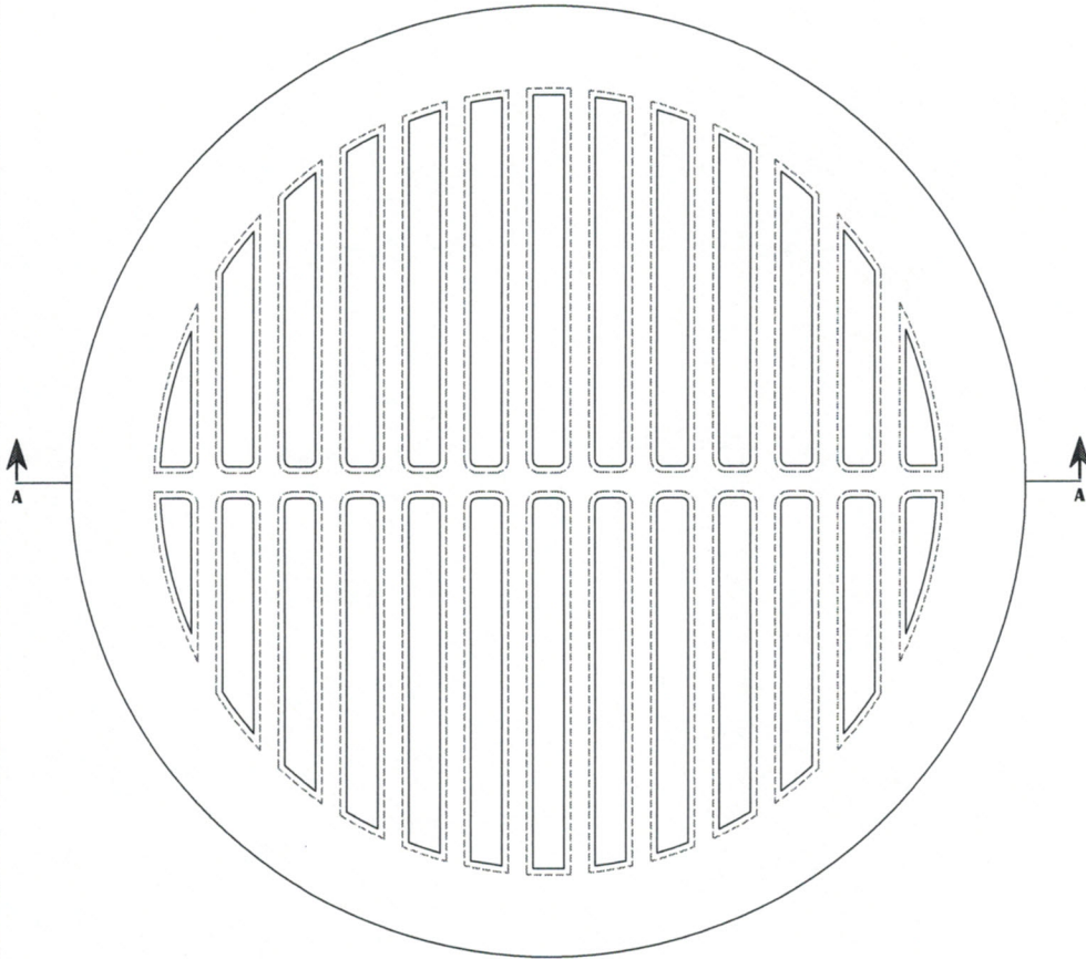
PLAN OF GRATE
